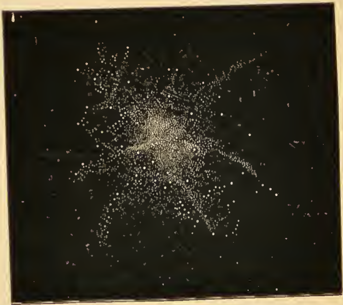
FIG. 87.—Old drawing of the cluster in Hercules.
